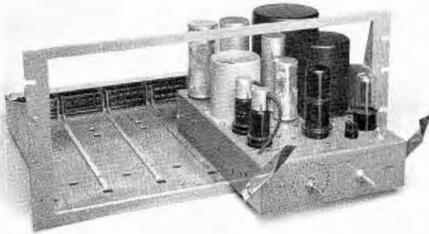
FIG. 6. With front panel of BR-2A removed, amplifiers easily slide into place. Guide strips on shelf insure proper positioning.
