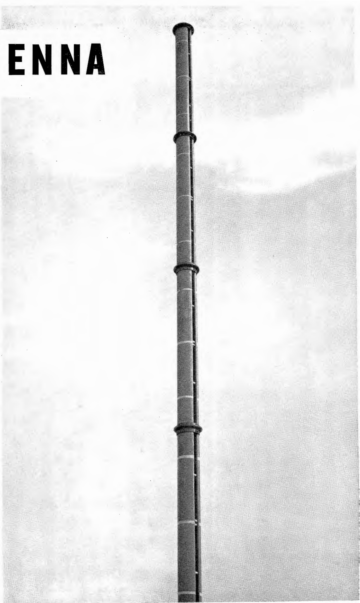
FIG. 2. (Right) Pylon sections may be stacked to provide high gain. Shown here is a four-section Pylon having a power gain of six. As many as eight sections (power gain of twelve) may be stacked in this manner. The structure is self-supporting, relatively light in weight.
