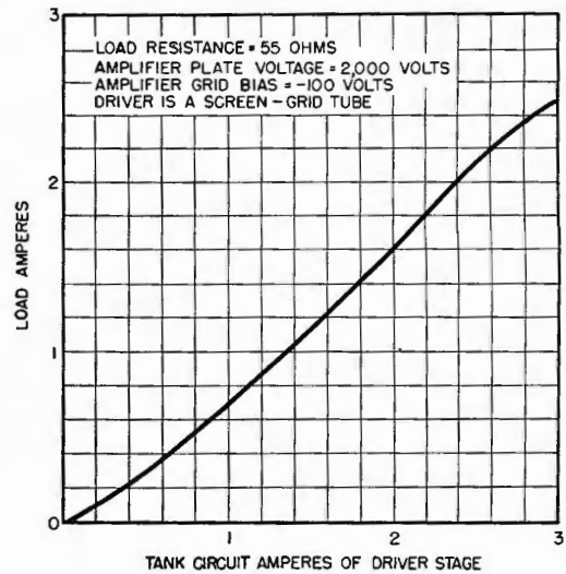
FIG. 6. Class-B power amplification characteristic of grounded-grid circuit.
