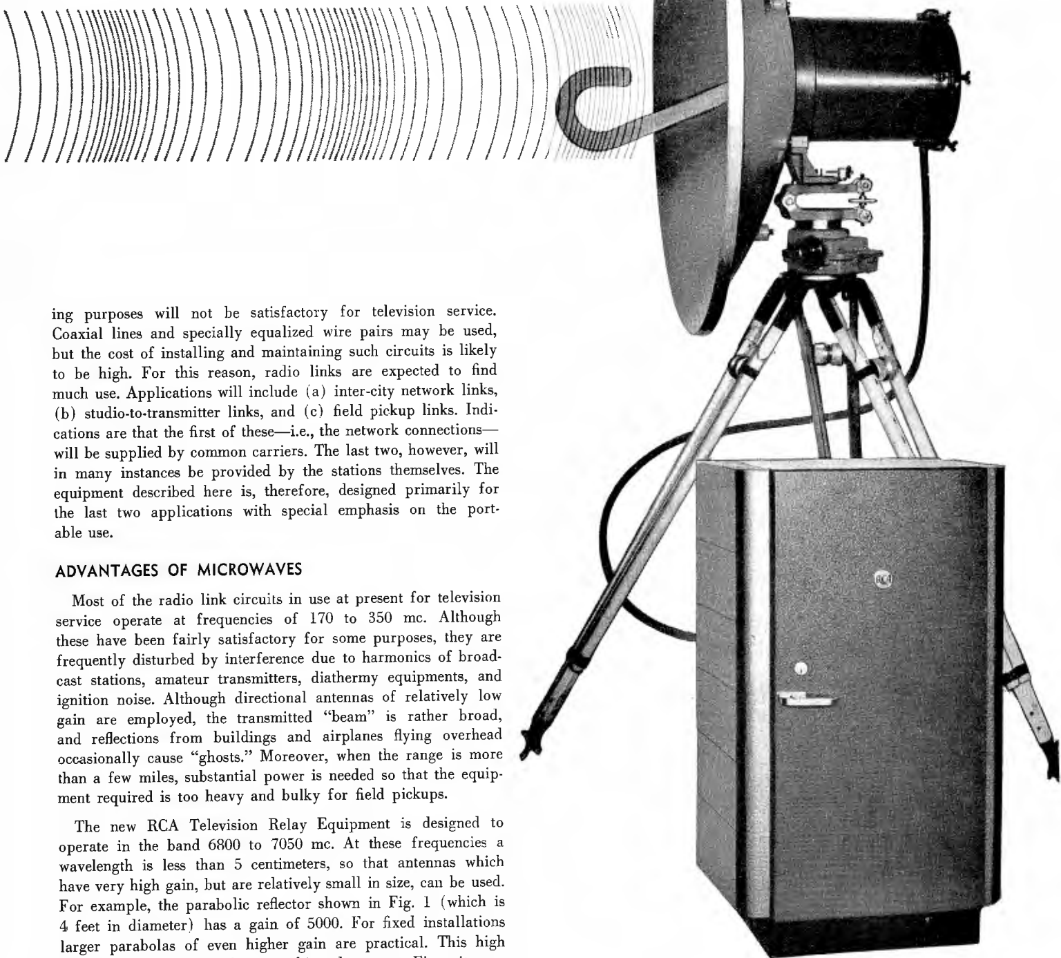
FIG. 2. This is the microwave receiving equipment. It consists of a parabolic antenna (identical to that at the transmitter), the receiver pre-amplifier, (in the cylindrical case attached to the rear of the parabola), the receiver control unit, and a power supply unit. The last two are mounted in the cabinet at the bottom. The control unit in a portable case is shown in Fig. 17.
