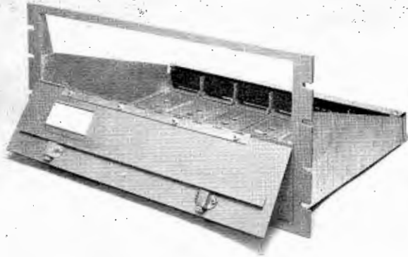
FIG. 4. BR-2A Shelf has front panel 8 \frac{3}{4} " high—is designed to mount on old-type open racks or new RCA cabinet racks.
