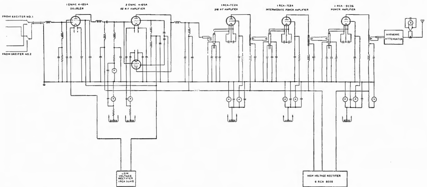
FIG. 2. (Above) Simplified schematic diagram of the RCA BTF-10B Transmitter, Schematic of the exciter was shown in BROADCAST NEWS No. 42 (January 1946) on Page 29.
