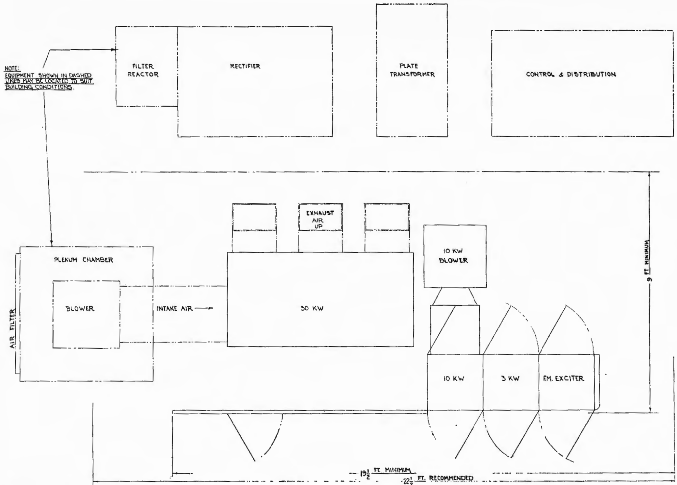
FIG. 1. Suggested floor layout for the BTF-50A Transmitter. The various component units may be arranged to suit the space available (see text).
